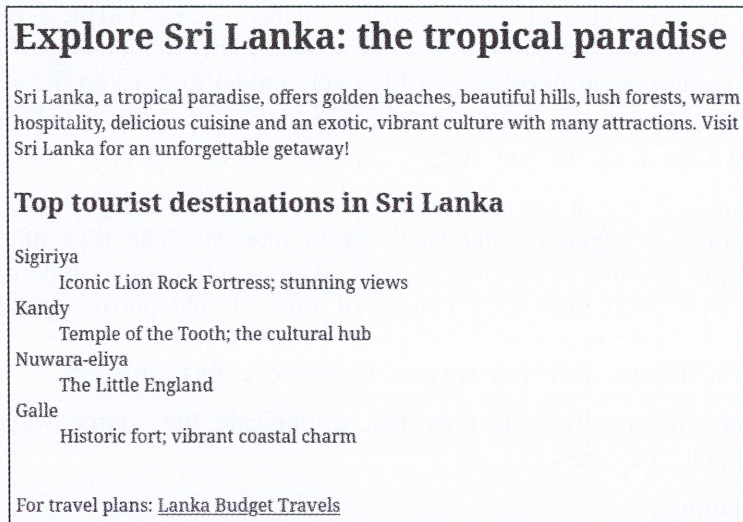
Figure 1: Web page
